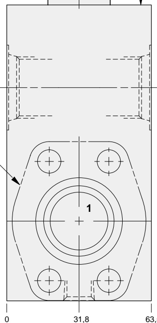
Normally Open Solenoid Valve
